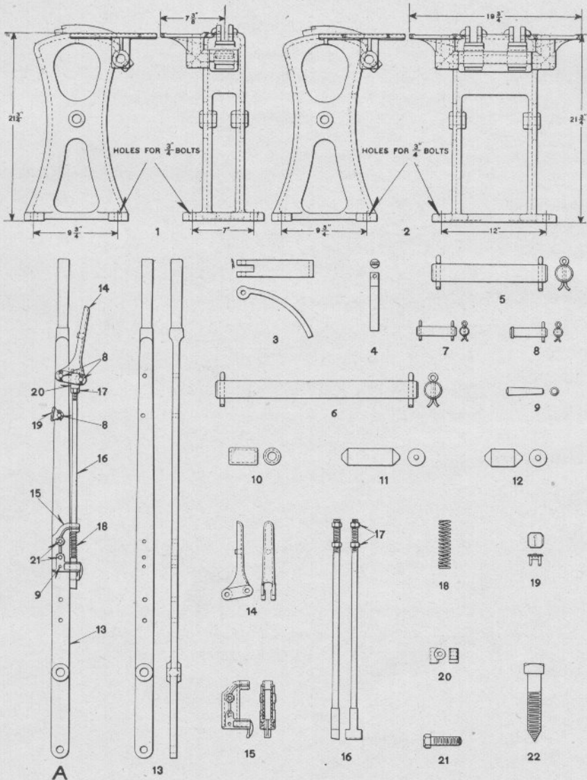
LEVERS, STANDS, TAPPETS, LOCKING DOGS, ETC. FOR DWARF INTERLOCKING MACHINE
